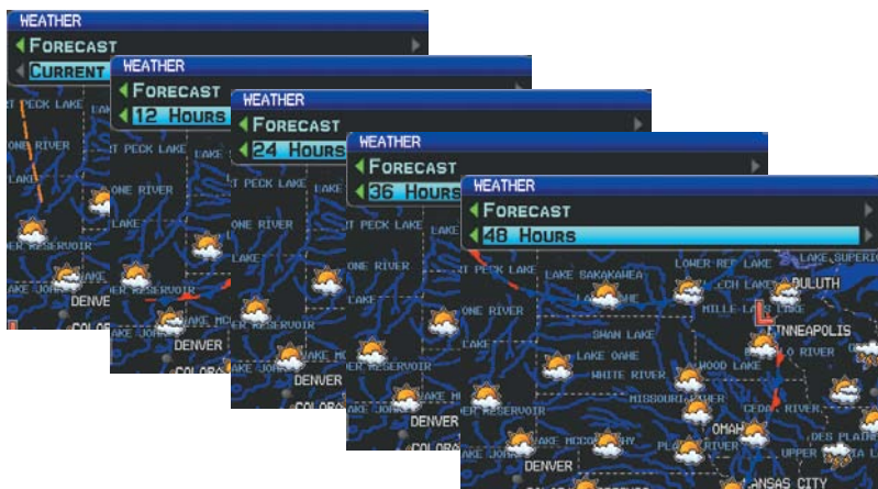
Forecast Data
