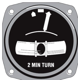
Turn and slip indicator showing a rate 1 turn to the right.
